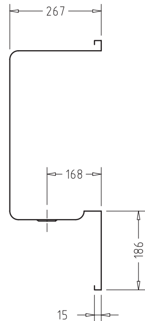
SECTION
